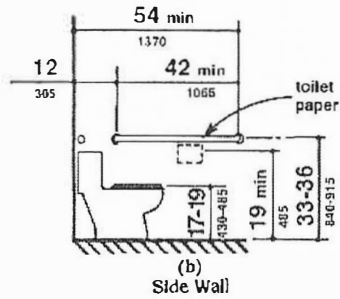
(b) Side Wall
