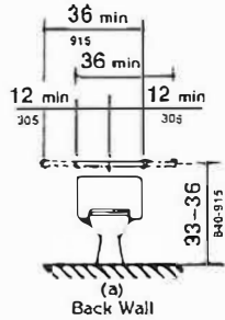
1. Grab bar at wc
