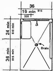
(b) Side Wall
