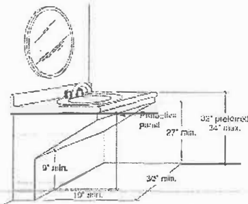
4. Ada compliant wash basin
